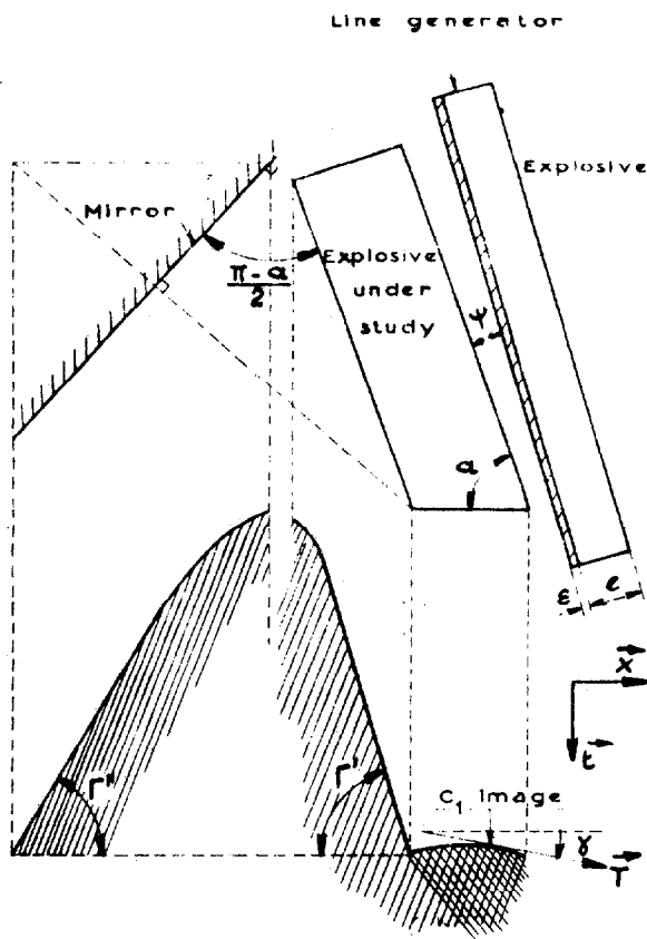
Fig 5 - Photographic arrangement
